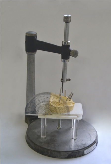
Figure 4: Full measuring apparatus setup. Analyzing rod attached to tool holder.
